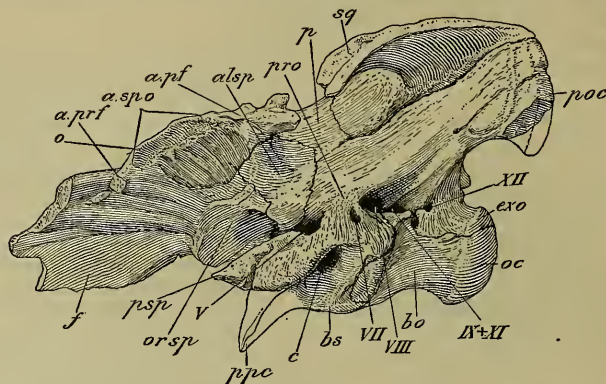
FIG. 10.—OBLIQUE SIDE VIEW OF THE POSTERIOR PART OF THE SKULL OF STEGOSAURUS SP. CAT. NO. 2274, U.S.N.M. \frac{1}{2} NAT. SIZE. alspr , ALISPHEOID; a.pf , ARTICULAR BORDER FOR POSTORBITAL; a.prf , ARTICULAR BORDER FOR PREFRONTAL; a.spo , ARTICULAR BORDER FOR POSTFRONTAL; bo , BASIOCCIPITAL; bs , BASISPHENOID; c , EXIT FOR CAROTID ARTERY; exo , EXOCCIPITAL; f , FRONTAL; o , ORBIT; oc , OCCIPITAL CONDYLE; orsp , ORBITOSPHENOID; p , PARIETAL; poc , PARI OCCIPITAL PROCESS; ppc , PROCESS FOR PTERYGOID; pro , PROÏTIC; psp , PRESPHENOID; sq , SQUAMOSAL; V, VII, VIII, IX, X, XI, AND XII, EXITS OF CRANIAL NERVES.
