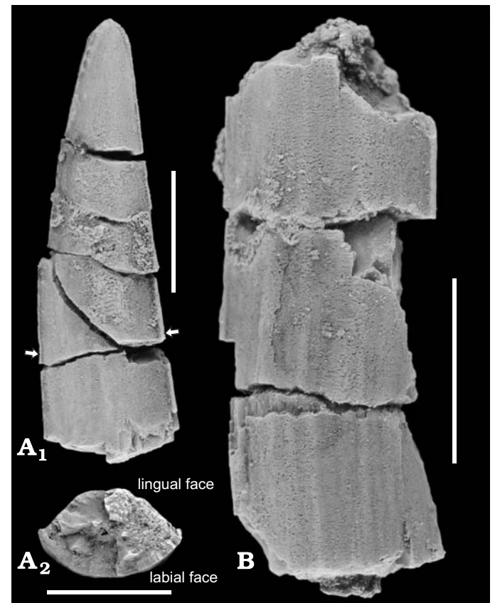
Fig. 4. Tooth of rebbachisaurid sauropod Demandasaurus darwini gen. et sp. nov. from Late Barremian–Early Aptian, Early Cretaceous of Tenadas de los Vallejos II, Spain. A. MDS-RVII,438, in lingual (A 1 ) and basal (A 2 ) views. B. Detail of the ornamentation of the tooth MDS-RVII,437, in lingual view. The arrows indicate the mesial and distal carinae. Scale bars 5 mm.
