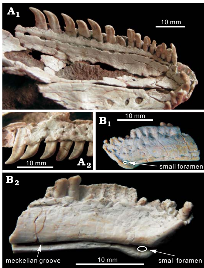
Fig. 3. A troodontid theropod Xixiasaurus henanensis gen. et sp. nov. (HGM 41HIII-0201; holotype), lower–middle Majiacun Formation (Upper Cretaceous: Coniacian–Campanian), Henan Province, China. A. Rostrum of skull in palatal ( A_1 ) and right lateral ( A_2 ) views. B. Anterior part of left dentary in lateral ( B_1 ) and medial ( B_2 ) views.
