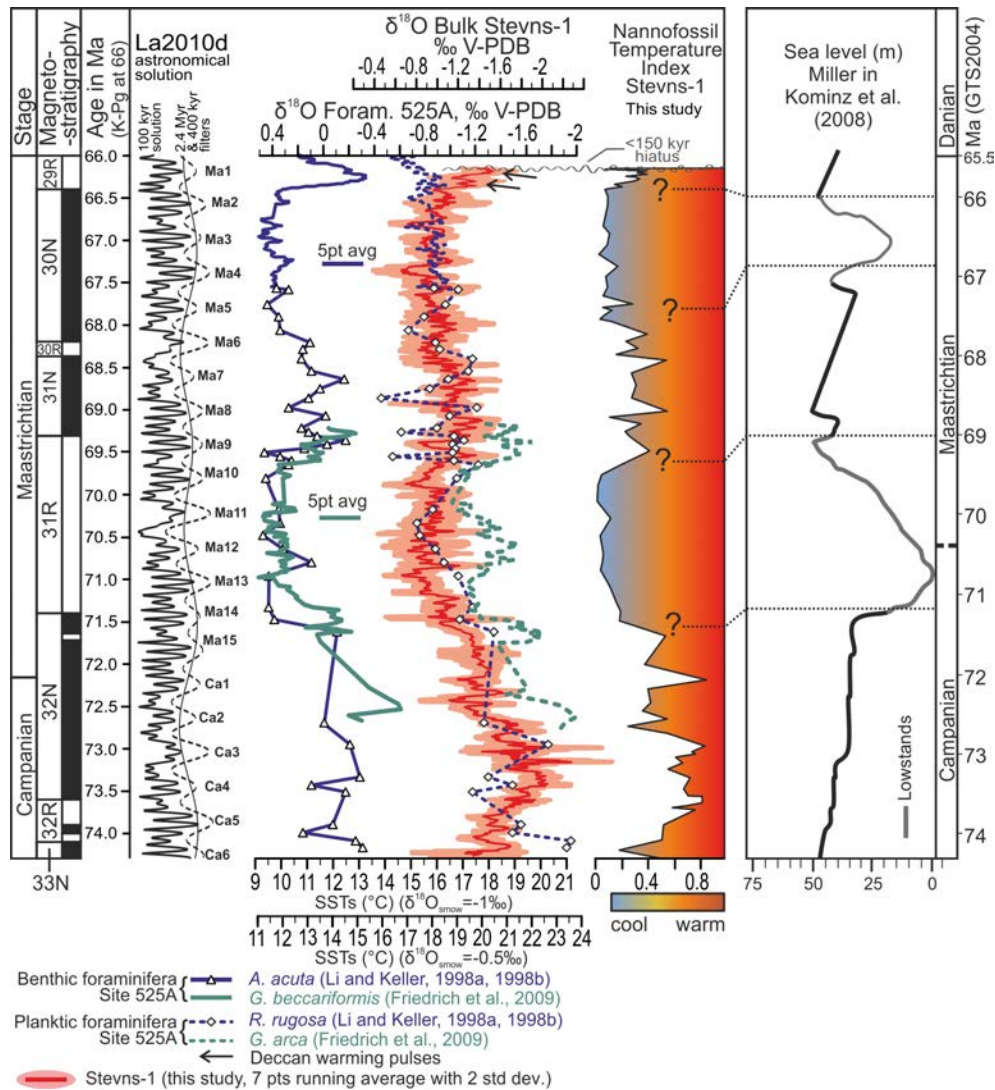
Figure 5. Stable oxygen isotope and calcareous nanofossil data of Stevns-1 compared to data on foraminifers of South Atlantic DSDP Site 525A. The age scale is based on the correlation of carbon isotope curves between Stevns-1, DSDP Site 525A and the astronomically calibrated ODP Site 762C. La2010d: astronomical solution from Laskar et al. (2011). Benthic and planktic foraminiferal stable isotope data from Li and Keller (1998a, b) and Friedrich et al. (2009).
